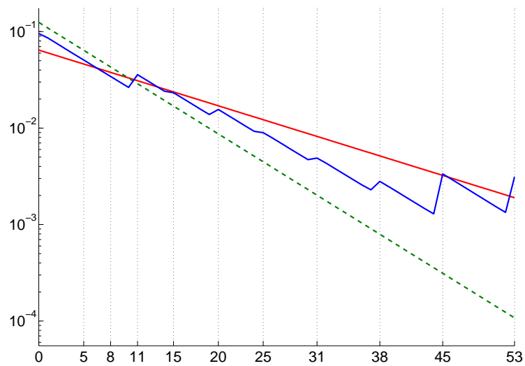
Figure 2: Cooling the cavity: 5000 interactions.
