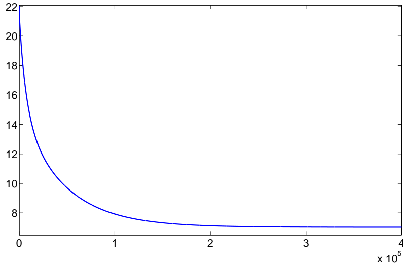
Figure 4: Cooling the cavity: average photon number.
