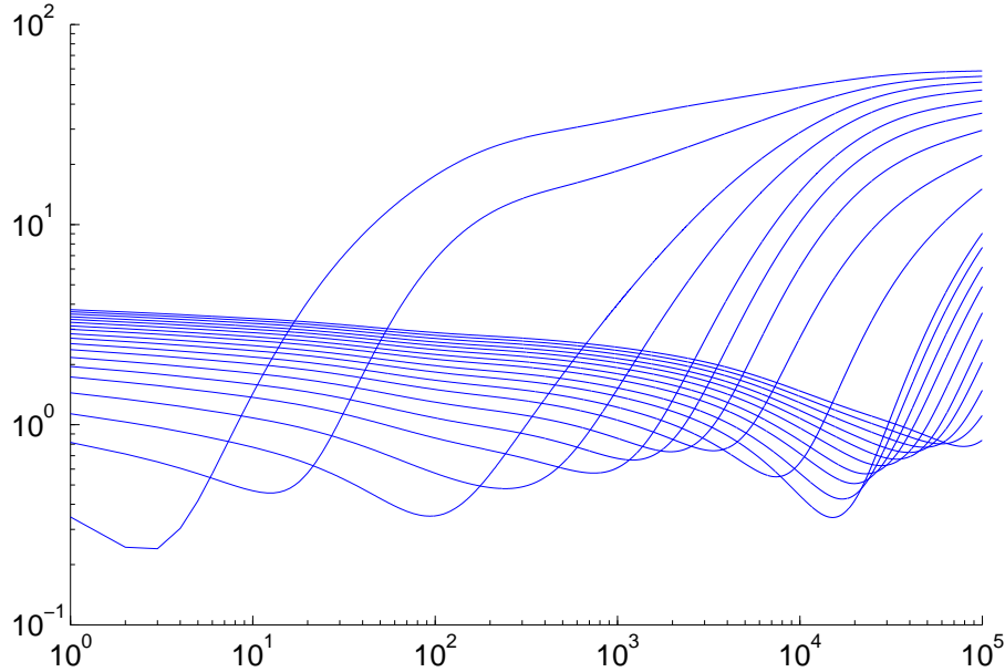
Figure 1: The metastable cascade (notice the log-log scale !).
