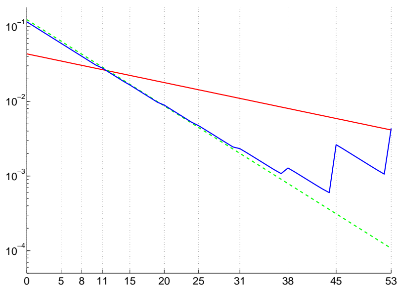
Figure 3: Cooling the cavity: 50000 interactions.
