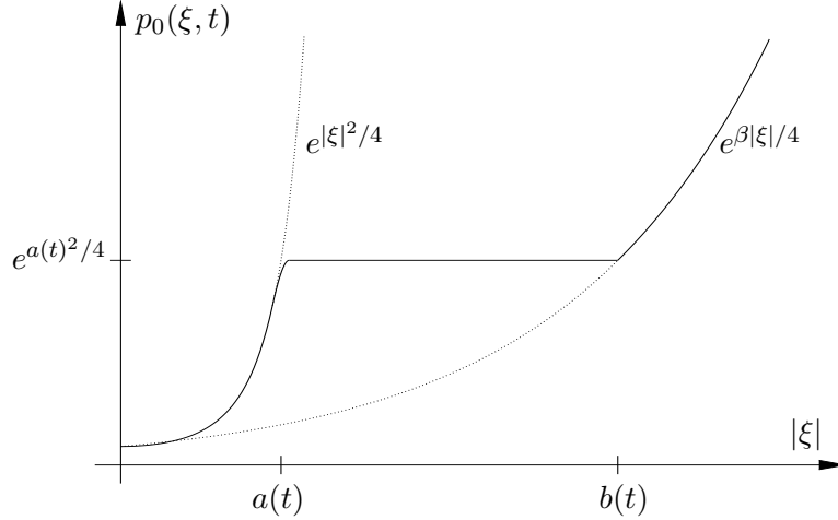
Fig. 1: The radially symmetric, time-dependent weight p_0(\xi, t) is represented as a function of |\xi| . The gradient of p_0(\xi, t) has a jump discontinuity at |\xi| = b(t) , but is Lipschitz continuous near |\xi| = a(t) .
