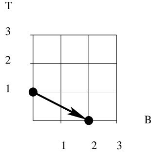
FIGURE 1. E_2 page of the spectral sequence.
