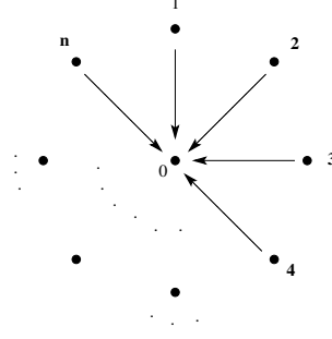
Figure 1: The quiver for a hyperpolygon space.
